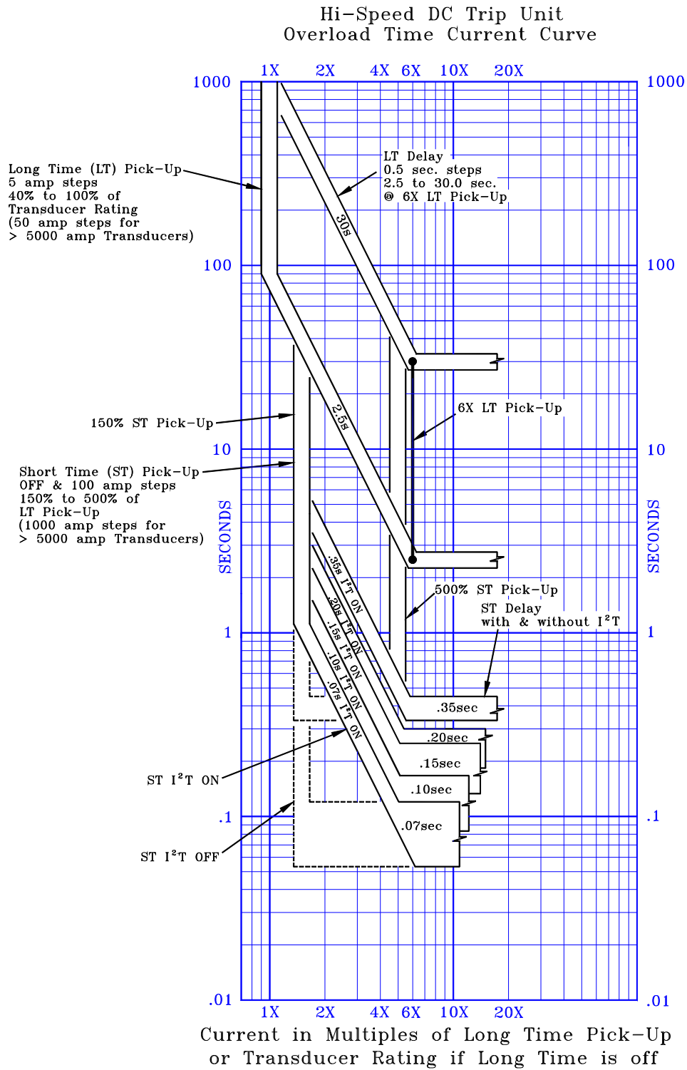
FIGURE 8 Non-Hi-Speed Trip Functions TCC
